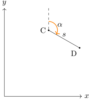
Figure 1.3: Azimuth \alpha and distance s measured from point C to point D to determined the coordinates of point D .
